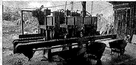
Reaserradora o multiple
